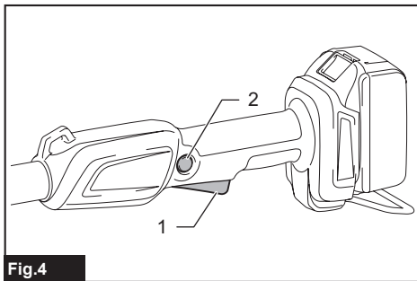
Fig.4 ► 1. Switch trigger 2. Lock-off button
