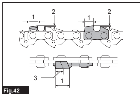
Fig.42 ► 1. Cutter length 2. Distance between cutting edge and depth gauge 3. Minimum cutter length (3 mm (1/8"))
